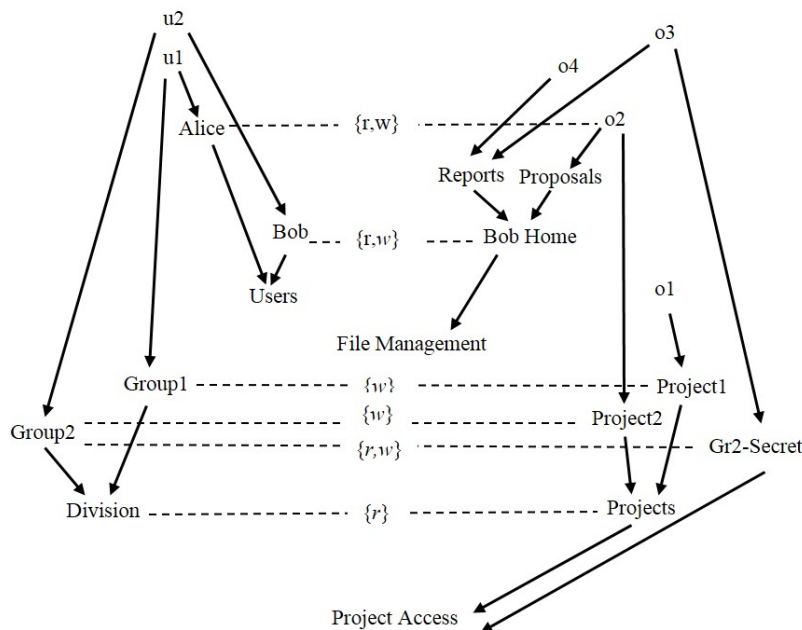
Figure 7: Graphs from Figures 6a and 6b in Combination
