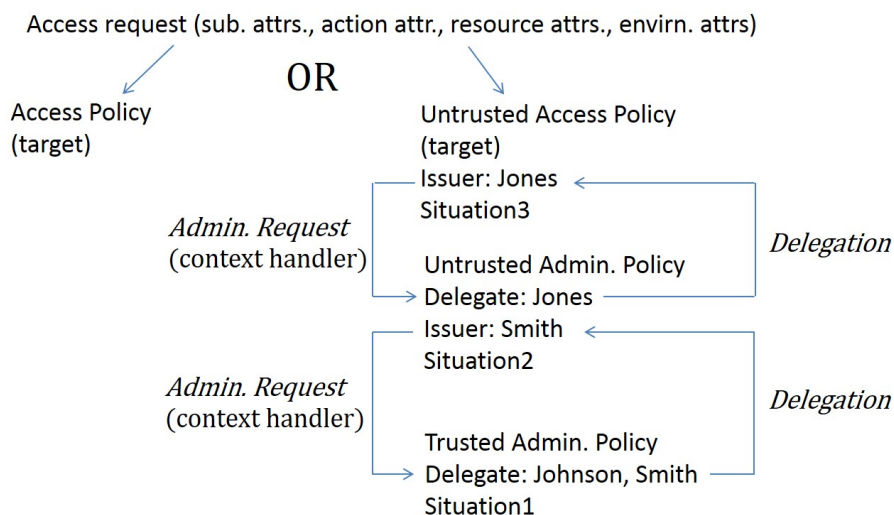
Figure 3: An Example of a Delegation Chain
