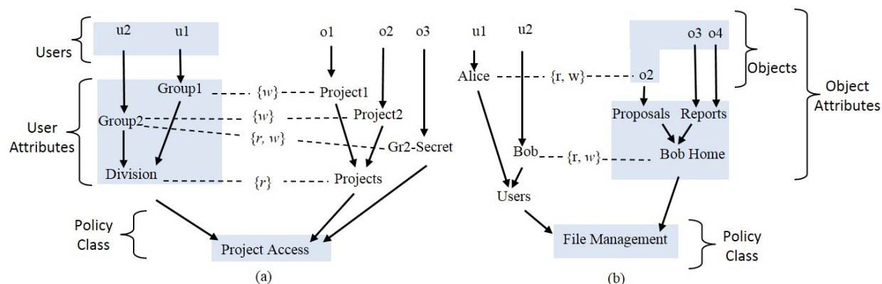
Figure 6: Two Example Assignment and Association Graphs
