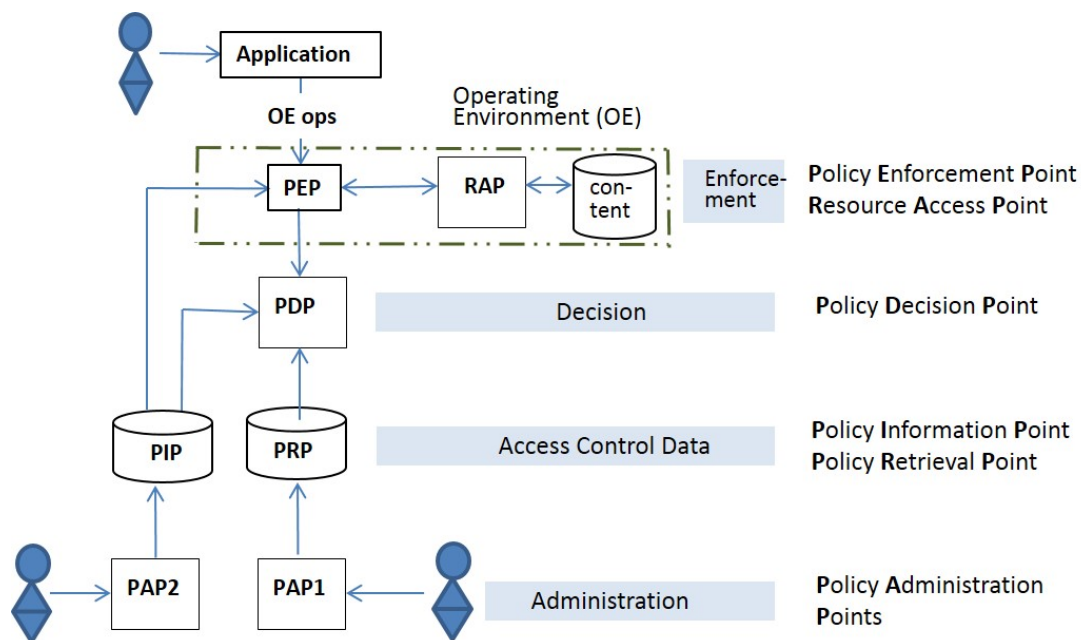
Figure 5: XACML Reference Architecture
