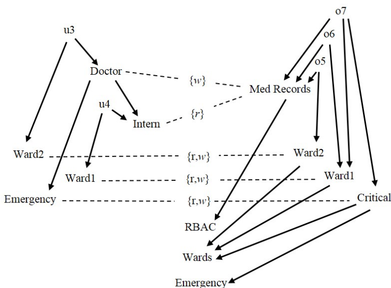
Figure 8: NGAC's Equivalent Expression of XACML Policy1
