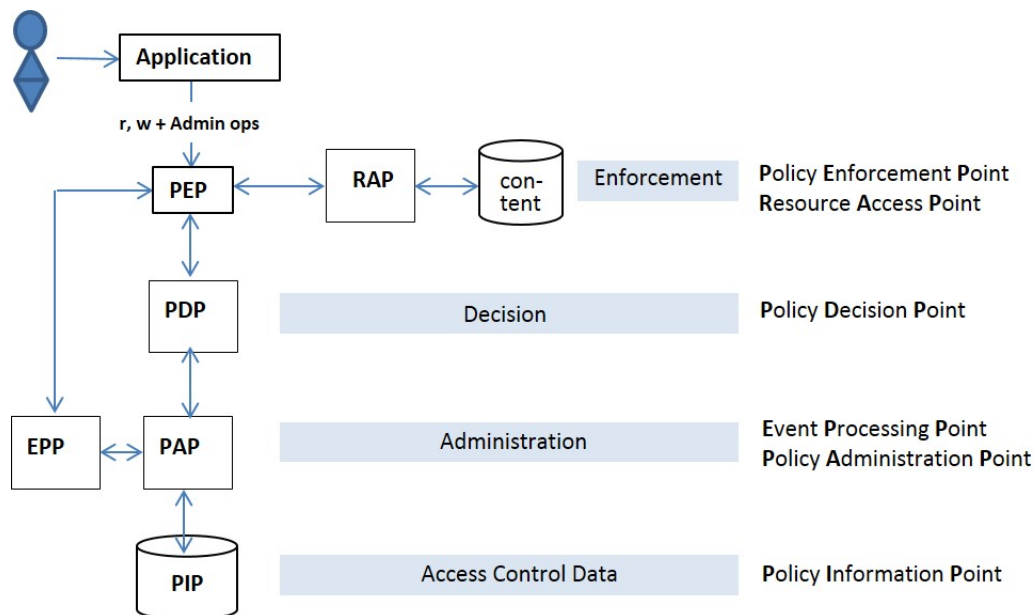
Figure 9: NGAC Standard Functional Architecture
