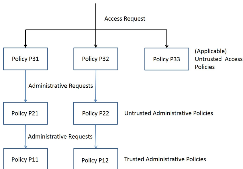
Figure 4: Utilizing Delegation Chains for Policy Evaluation
