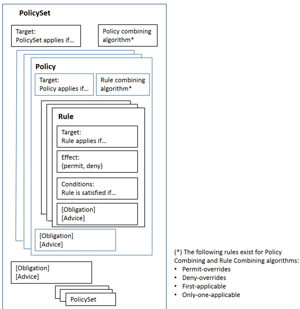
Figure 2: XACML Policy Constructs
