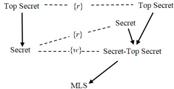
Figure 10: NGAC's Partial Expression of TCSEC MAC
